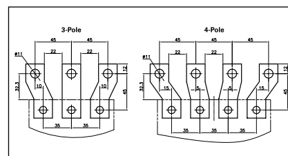
Figure 6. Terminal Spreaders
