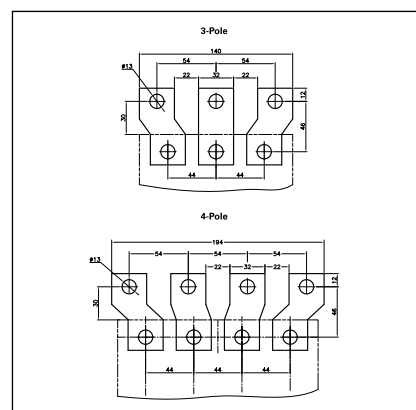
Figure 7. Terminal Spreaders
