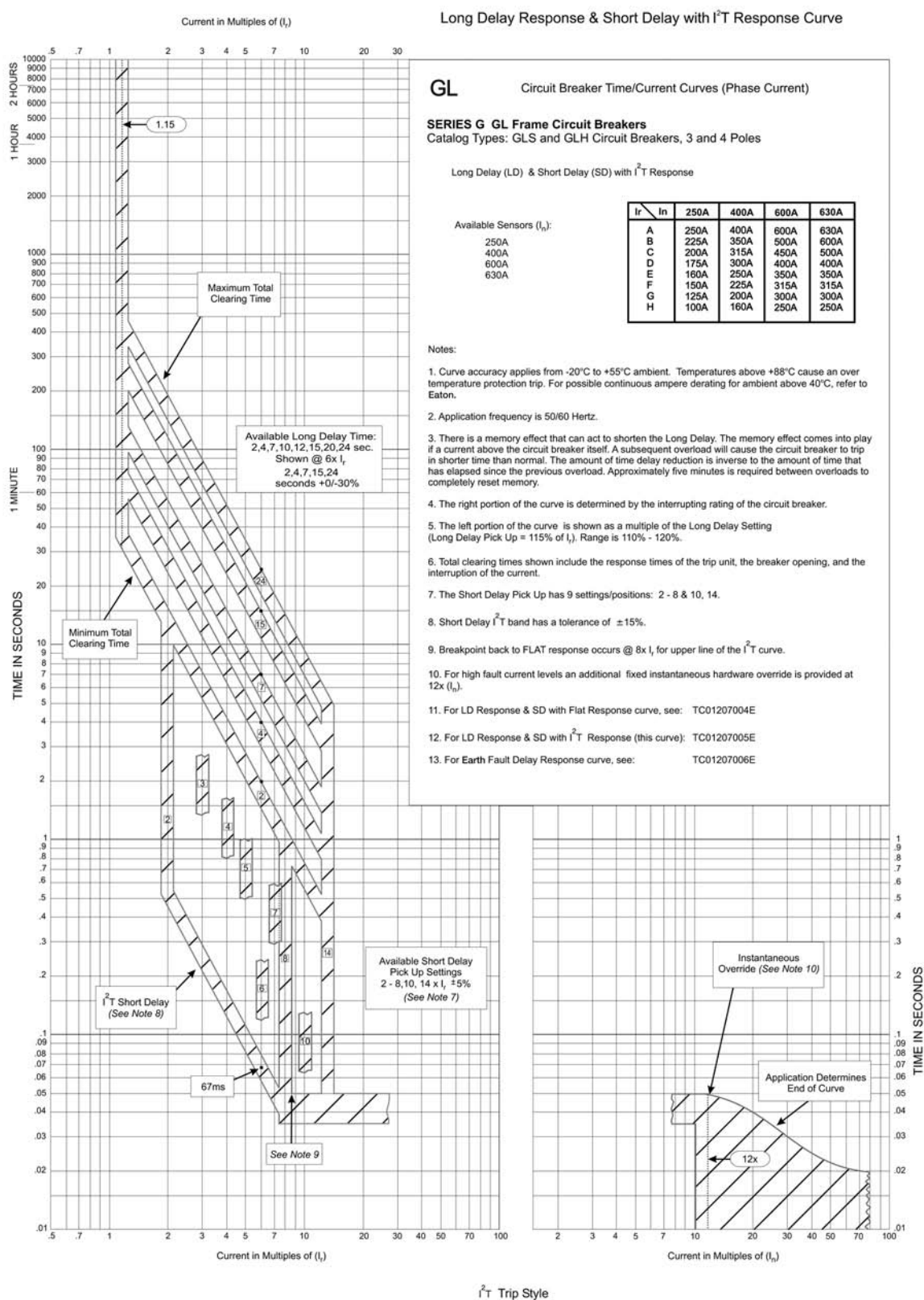
Figure 18. GL Electronic Trip Unit Long Delay Response and Short Delay with I 2 T Response Curve
