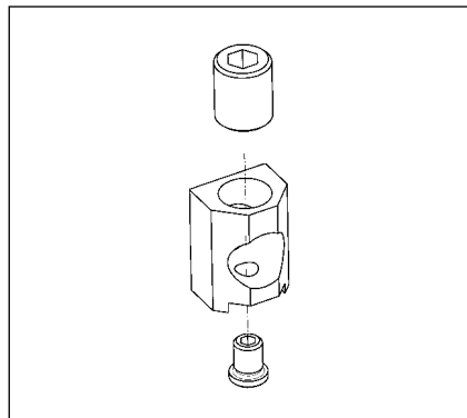
Figure 5. Standard and Optional Pressure Type Terminal TA250FJ/TC250FJ
