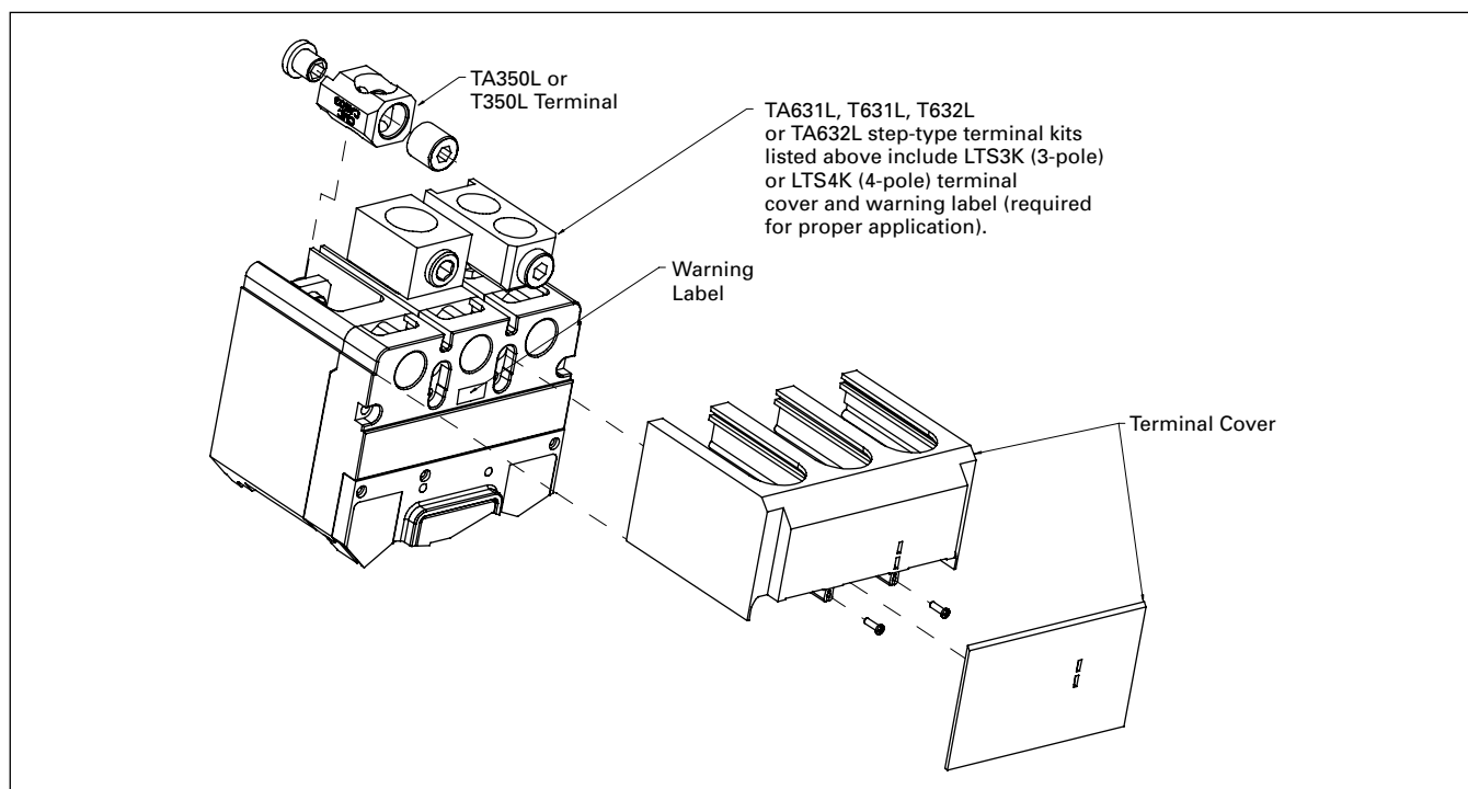
Figure 8. Terminals and Terminal Cover for the GL Breaker — Includes LTS3K (3-Pole) or LTS4K (4-Pole) Terminal Covers
