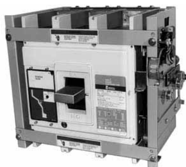
Drawout Cassette
