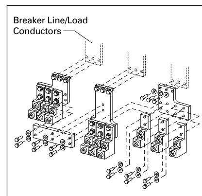
Figure 10. TA2000RD Wire Terminal
