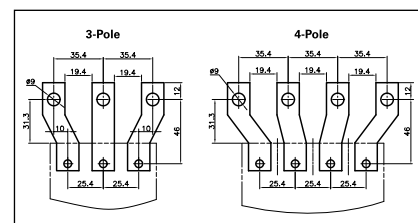
Figure 3. Terminal Spreaders
