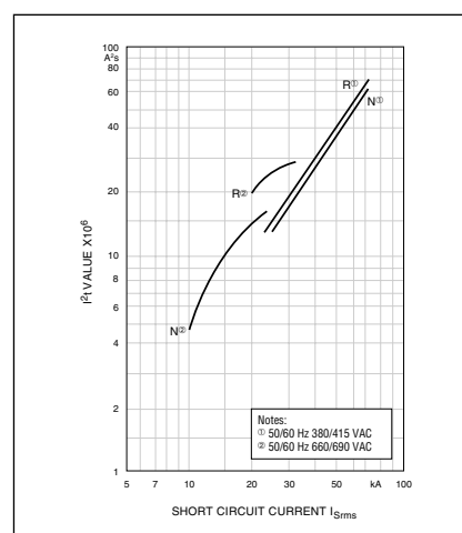
Figure 28. Maximum I^2t Values for GN to GR, 50/60 Hz 600/660/690 Vac
