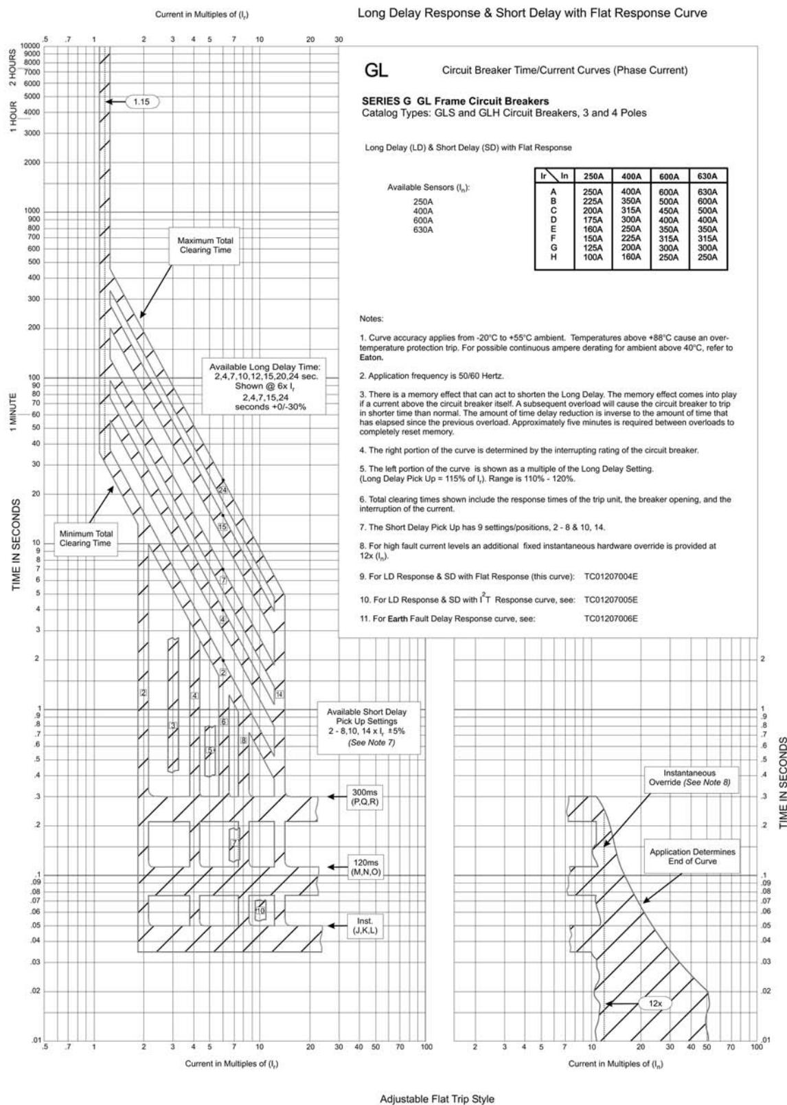
Figure 19. GL Electronic Trip Unit Long Delay Response and Short Delay with Flat Response Curve
