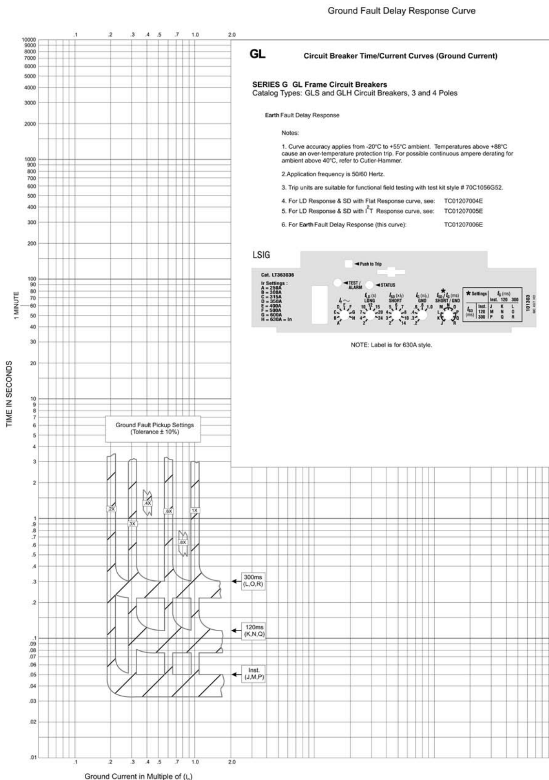
Figure 20. GL Electronic Trip Unit Earth Fault Delay Response Curve
