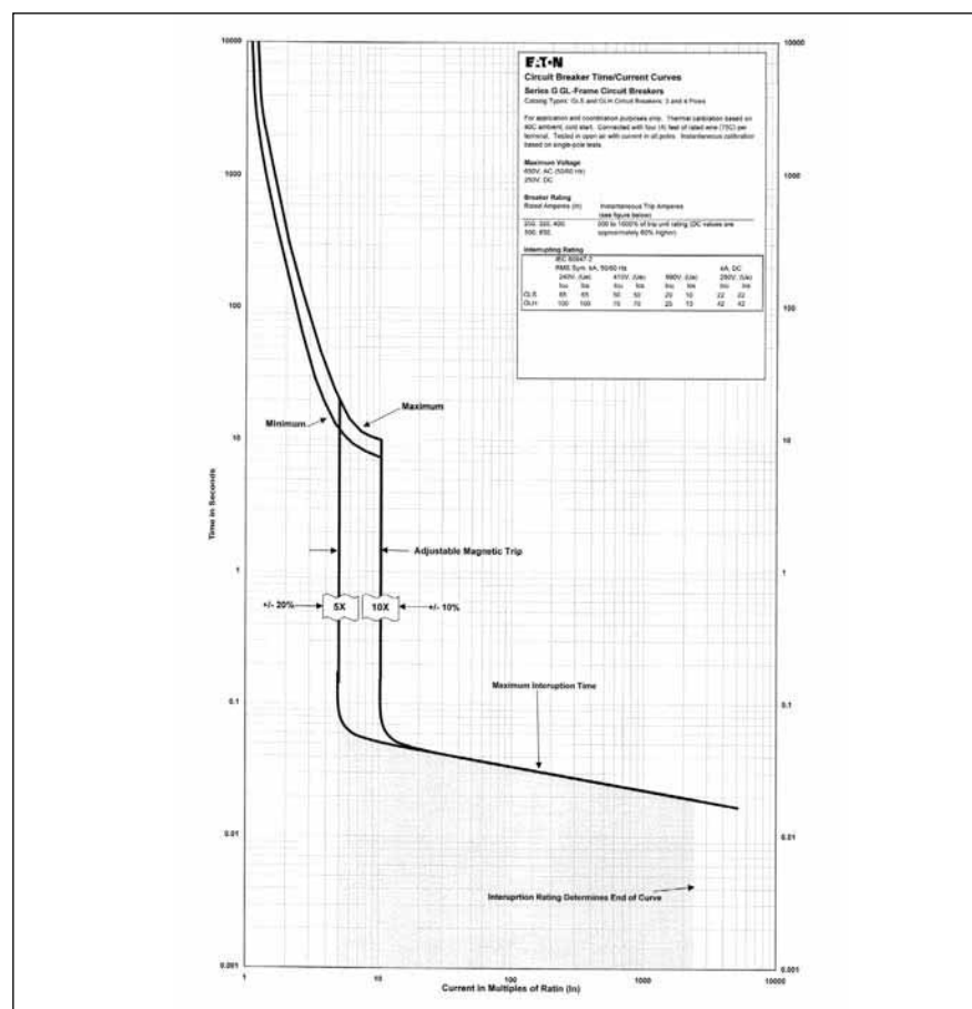
Figure 17. GL Time Current Curve for Thermal Magnetic Trip Units
