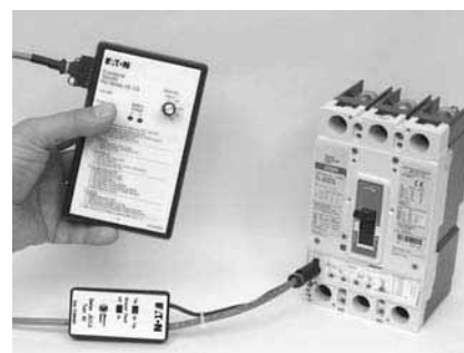
Digitrip 310+ Test Kit Shown with GJ MCCB
