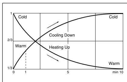
Figure 14. Tripping Time Characteristics (Thermal Memory)
