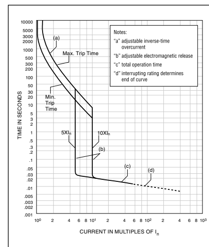
Figure 16. GJ Time Current Curve for Thermal Magnetic Trip Units
