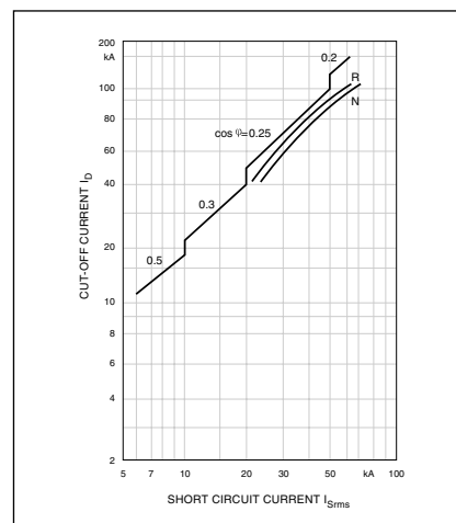
Figure 27. Current Limiting Characteristics I_p for GN to GR, 50/60 Hz 380/415/480 Vac
