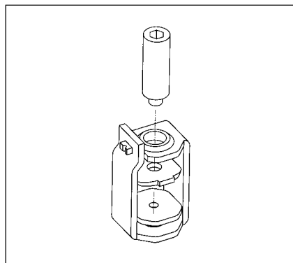
Figure 4. Standard Pressure Type Terminal T250FJ
